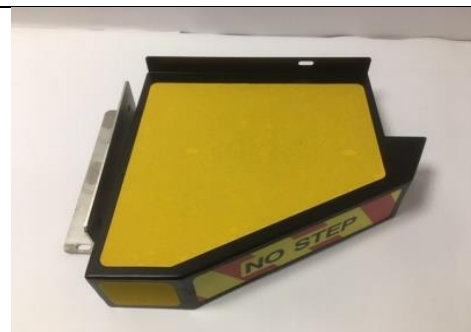
AP part no: DUC-0033-S Fiat Rear Step O/S Corner 'No Step' Platform (with fitting bracket) BIN Code 4711
