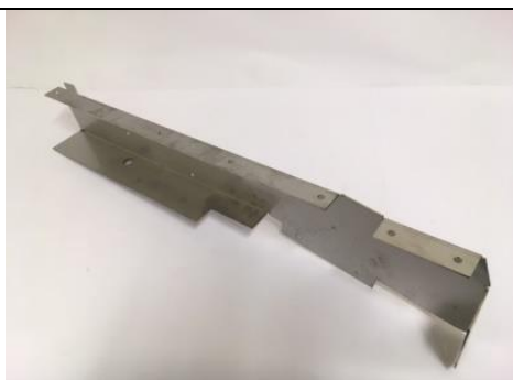
AP part no: RMP-0131-S Renault MK2 Floor-Pan Infil Panel/Mounting Bracket N/S
